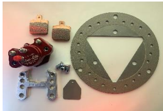
410-7200 1-T-250-9875-3 Rotor-Titanium-Solid .250" x 9.875" - 3 Bolt, 3-980-6000 Rotor Bolts, 1-140-1005/140-1006 100 Series Caliper - Floating Mount (1)-1.625" or 1.5" Piston, 1-930-0255 Caliper Bracket - Left Front Sprint with (2) .220" Spacers, 2- UL-104 Pad - Left Front Sprint 589A Compound, 1-170-0104 Heat Shield-
