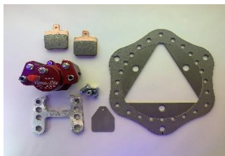
410-7300 1-CW-250-9875-3 Rotor-Steel-Scalloped-Solid .250" x 9.875" - 3 Bolt, 3-980-6000 Rotor Bolts, 1-140-1005/140-1006 100 Series Caliper - Floating Mount (1)-1.625" or 1.5" Piston, 1-930-0255 Caliper Bracket - Left Front Sprint with (2) .220" Spacers, 2-UL-104 Pad - Left Front Sprint 589A Compound, 1-170-0104 Heat Shield - Titanium - .065' Thick
